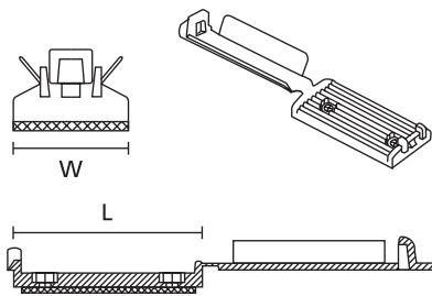
Flat Ribbon Cable Mounts - FKH-Series.
