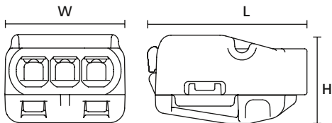
HelaCon Releasable, vista frontal
